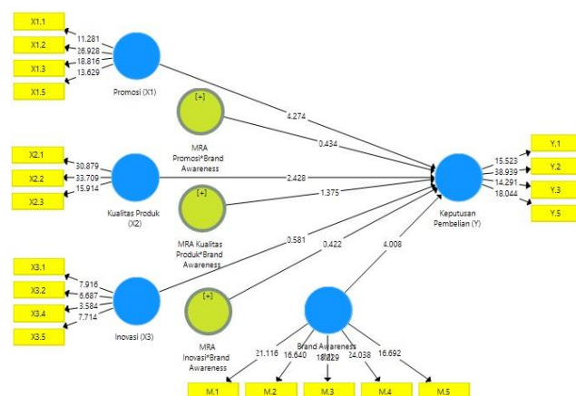
Figure 3. Output Bootstrapping
