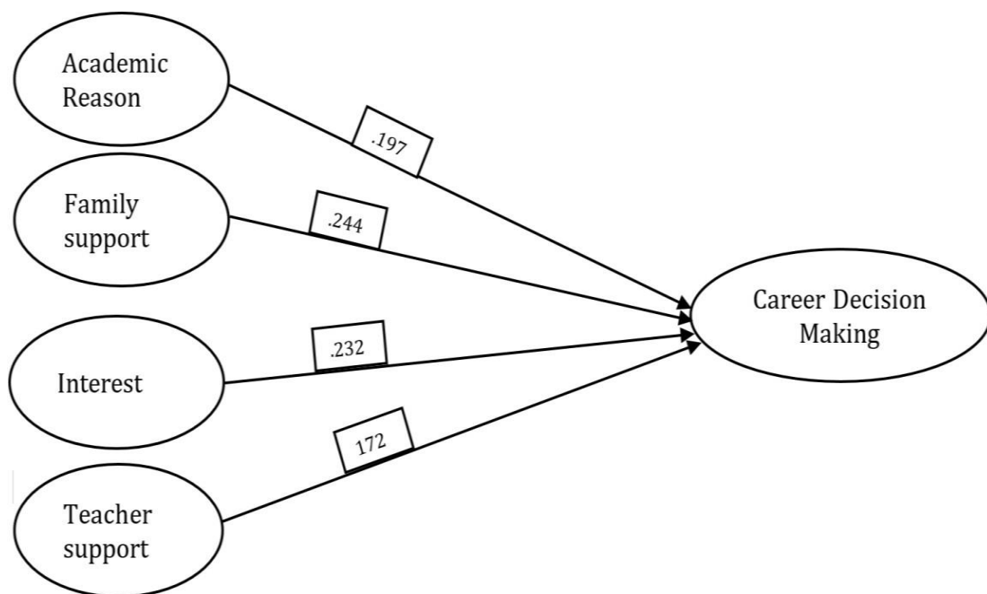
Figure.1: Research framework
